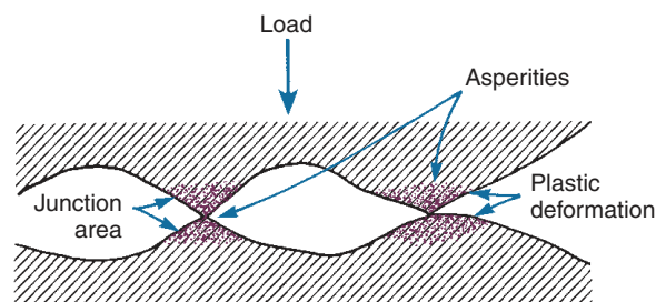
• Fig. 9.25 When two solid surfaces are pressed together or one slides over the other, real contact occurs only at a limited number of small spots, called asperities , that represent the peaks of surface irregularities. These junctions shear as sliding occurs, and the force to produce this plastic deformation of the surface irregularities is the frictional resistance. (Redrawn from Jastrzebski ZD. The Nature and Properties of Engineering Materials . 3rd ed. New York: Wiley; 1987.)
